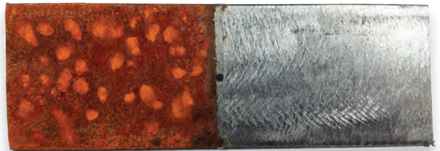
3/16" inch thick bare steel. Right side brushed with Rust Pro and wiped off. Steel exposed to open air (67°F, 63% humidity) and muriatic acid for 24 hours.
